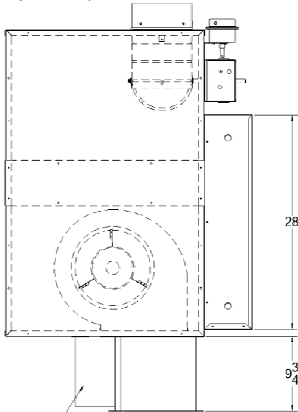
Heater Rack Access Cover
