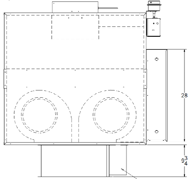
Heater Rack Access Cover
