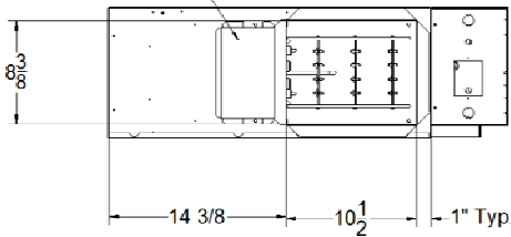
Heater Rack Access Cover
